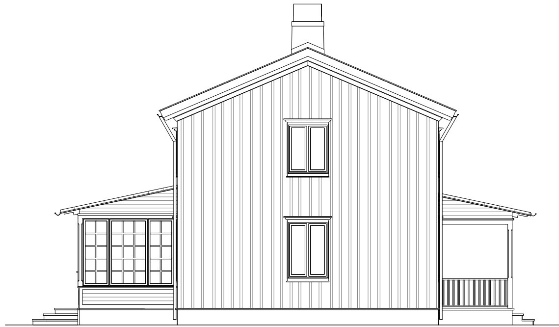
Fasad gavel, Hustyp 1
