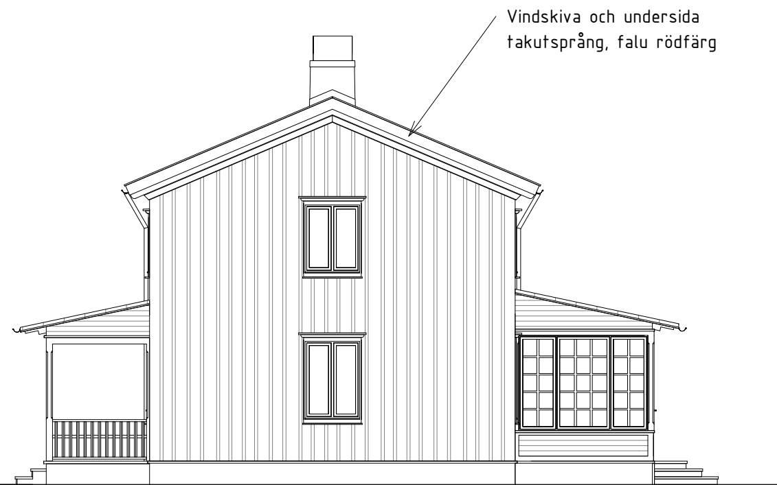
Fasad gavel, Hustyp 2
