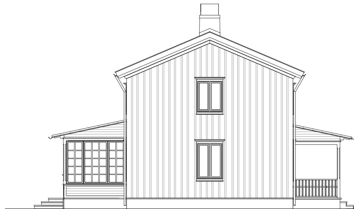
Fasad gavel, Hustyp 2
