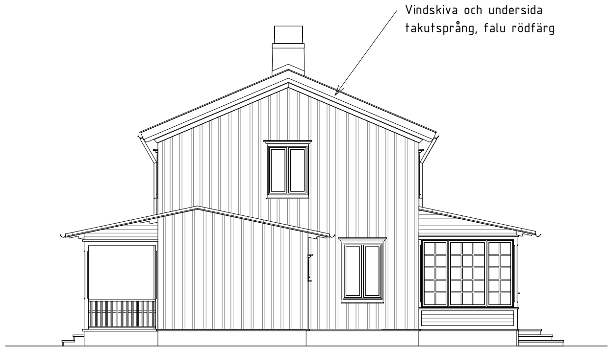
Fasad gavel, Hustyp 1
